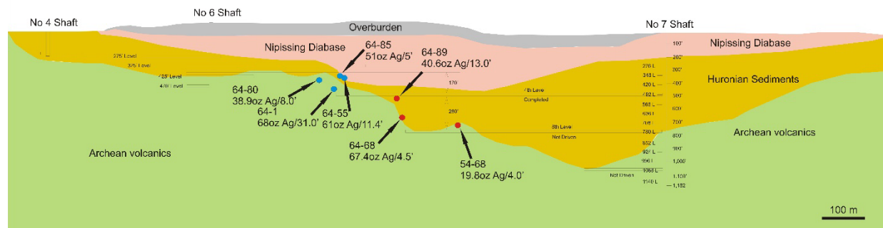
Langis Mine - Cross Section
