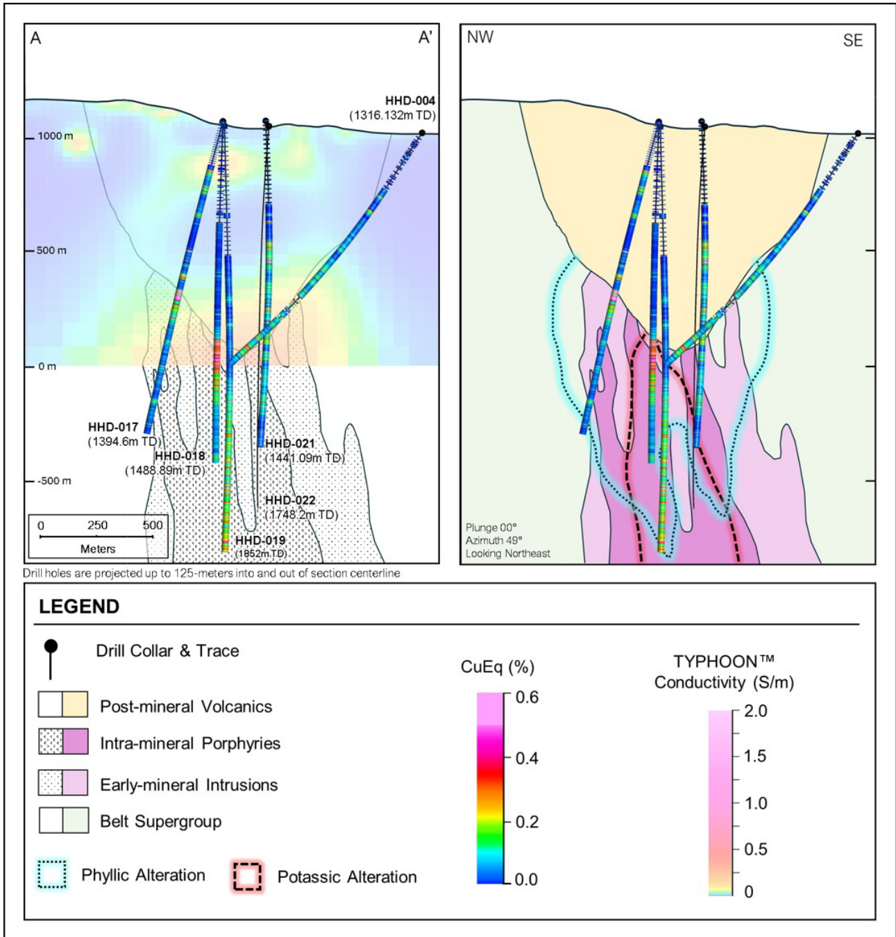
Figure 2. Cross-section A to A' at the Hog Heaven Project, looking northeast, of drilling at the Battle Butte Porphyry, showing Typhoon™ conductivity (left), drill holes, assay results, and simplified geology and alteration (right).
