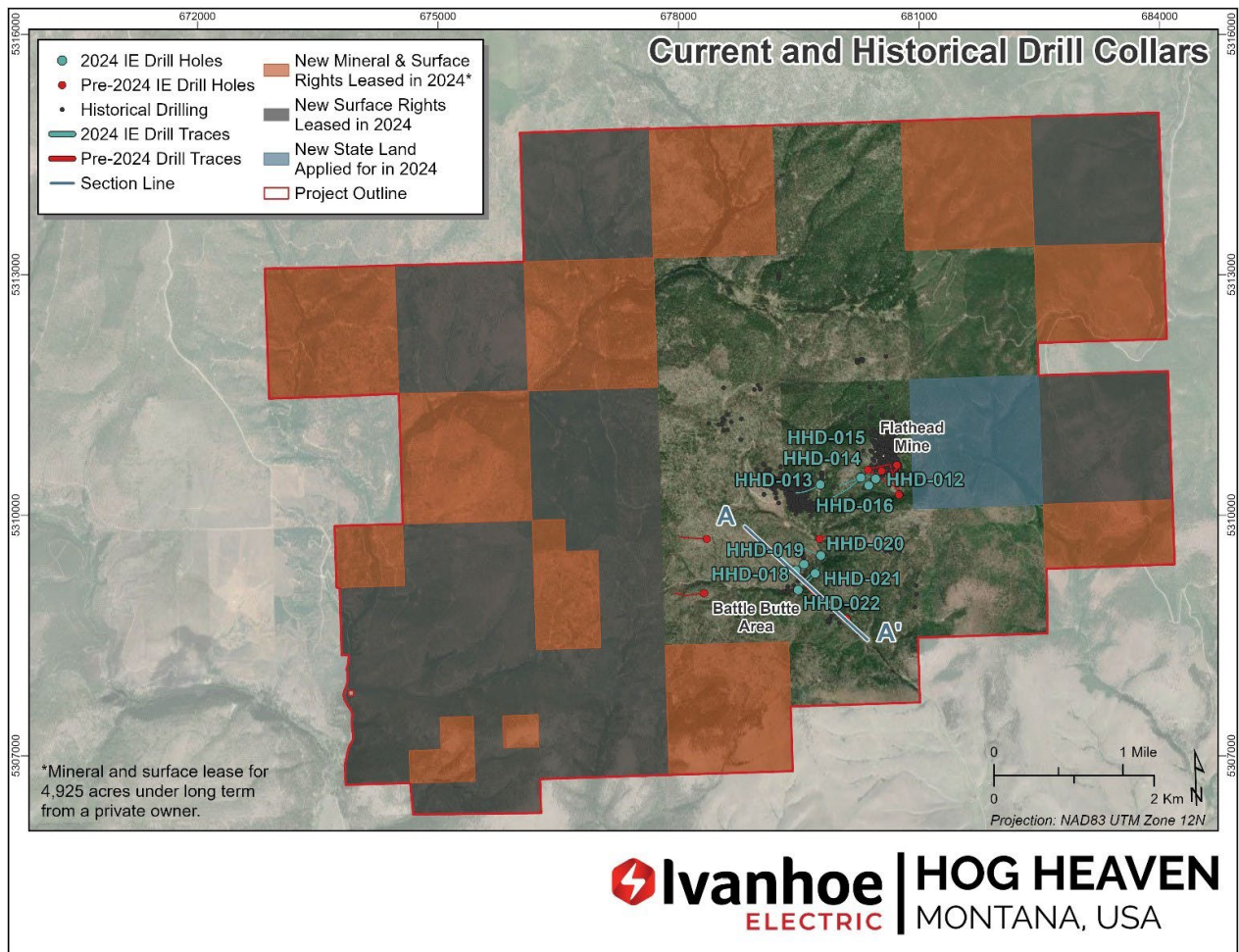
Figure 1. Plan view map of the Hog Heaven Project showing drill holes and their traces from the 2024 exploration program, newly leased land, and the location of cross-section A to A'.
